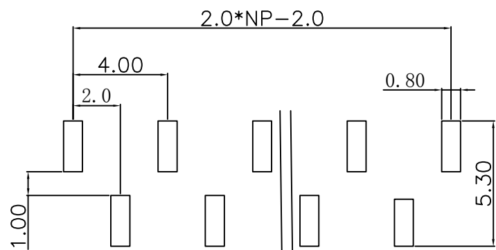
PCB LAYOUT
