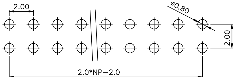
PCB LAYOUT
