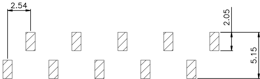
PCB LAYOUT
