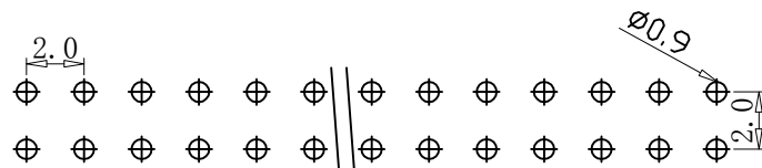
PCB LAYOUT
