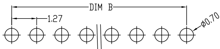
PCB LAYOUT
