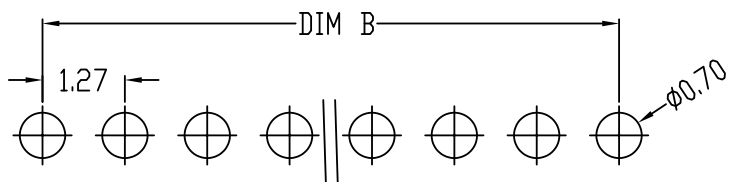
PCB LAYOUT
